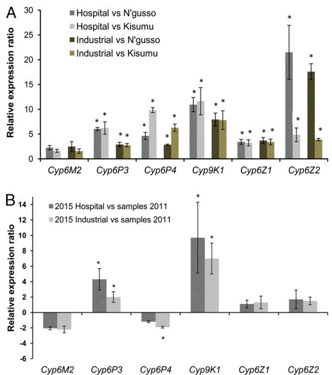
Fig. 4. Expression analysis of selected P450s by qPCR. (A) qPCR comparisons of selected P450 transcripts between hospital 2015 and industrial 2015 An. gambiae field populations from Bioko vs. the two susceptible laboratory colonies (N'gusso, Kisumu). Error bars represent the SE based on four biological replicates. Asterisk indicates a statistically significant difference in expression levels between the tested samples (Mann–Whitney U test, P < 0.05 ). (B) Comparison of P450 transcript expression levels between field-caught populations in 2015 (hospital and industrial) vs. samples collected in 2011. Error bars represent the SE based on four biological replicates. Asterisk indicates a statistically significant difference in expression levels between the tested samples (Mann–Whitney U test, P < 0.05 ).
