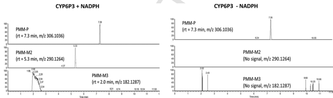
Fig. 3. Extracted ion chromatograms [M + H]^+ from CYP6P3 membranes. Pirimiphos-methyl parent (PMM—P) 7.3 min ( m/z 306.1036) observed in the presence (+) and absence (–) of NADPH. Metabolites pirimiphos-methyl oxon (PMM-M2) 5.26 min (290.1264) and 2-diethylamino-6-methyl-4-hydroxy-pyrimidine (PMM-M3) 2.0 min ( m/z 182.1287) observed in the presence of NADPH. Signals within the extracted ion chromatograms at different retention times correspond to low level background ions and/or electronic spikes.
