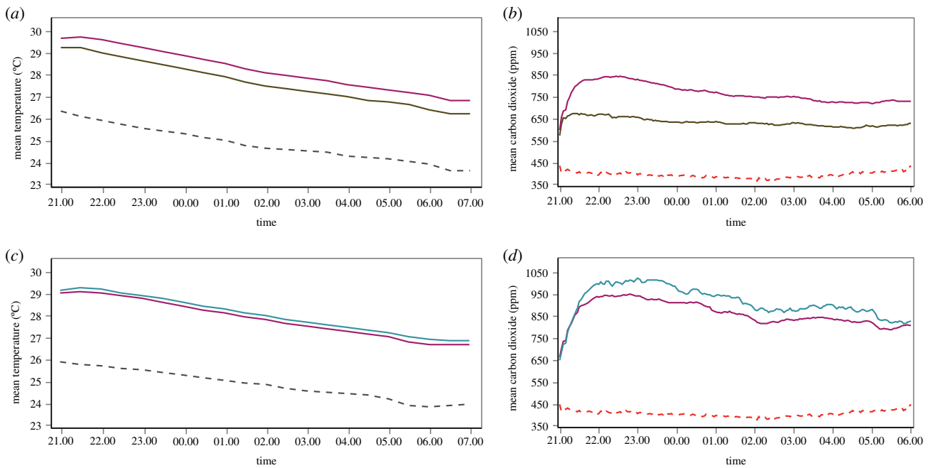
Figure 4. Nocturnal indoor and outdoor temperature (a,c) and indoor CO 2 concentrations (b,d) in screened and unscreened houses. Magenta lines, houses with screened windows and solid doors. Green lines, houses with screened windows and doors. Blue solid lines, houses with no windows and solid doors. Black broken lines, outdoor temperature. Red broken lines, outdoor CO 2 concentration. All measurements were made in year 2, apart from outdoor CO 2 , which was made in year 1.
