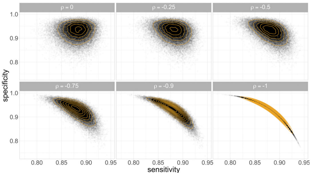
Figure 1. Scatterplots showing the bootstrapped values of sensitivity and specificity for different strengths of dependence (from independence to perfect correlation) between sensitivity and specificity. The empirical kernel density estimate for the bivariate distribution in each case is shown as orange contour lines.
