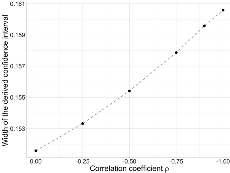
Figure 2. Width of the estimated confidence interval as a function of increased strength of the negative correlation between sensitivity and specificity.
