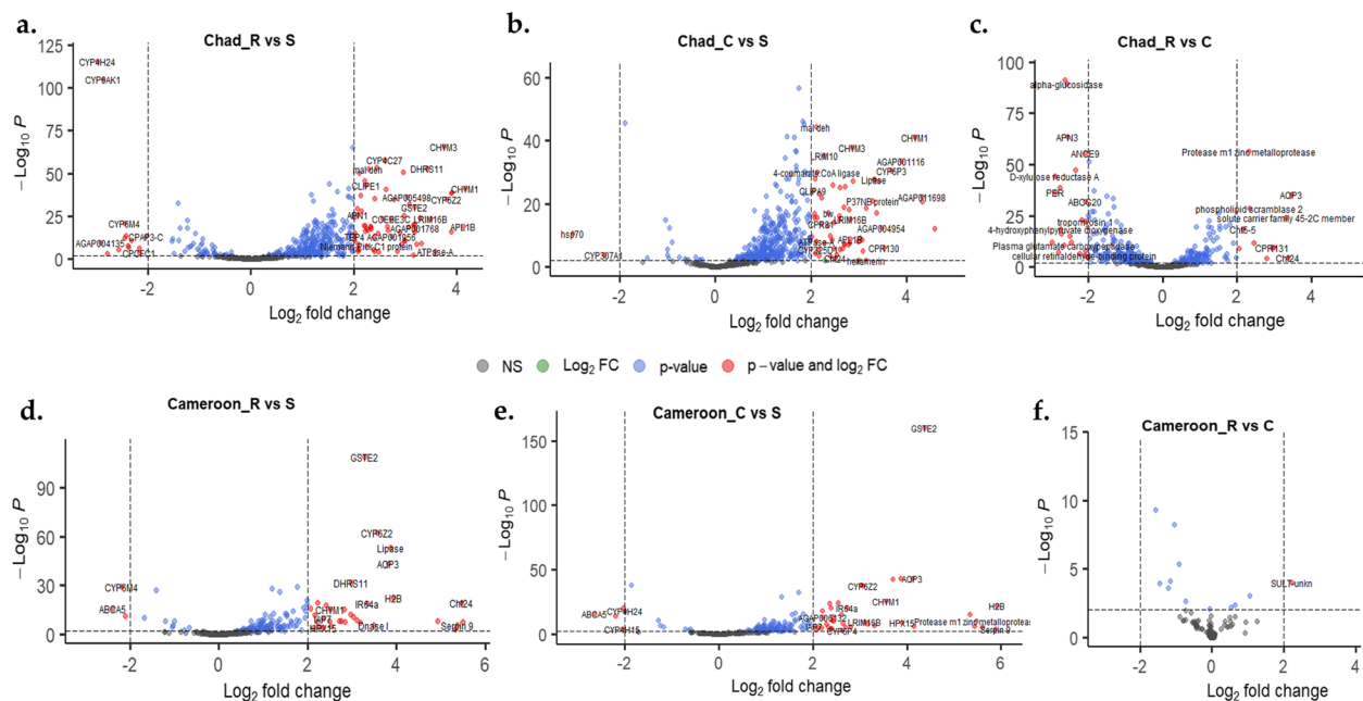
Fig. 2. A volcano plot of differentially expressed genes showing fold changes and significance in R-S, C-S and R-C comparisons, for Chad and Cameroon populations of An. coluzzii . The plot depicts the top upregulated and the top downregulated genes for each comparison with several genes including chymotrypsins, a malate dehydrogenase, an aquaporin, CYP450s (particularly CYP6Z2 ), a glutathione S-transferase ( GSTe2 ) and a lipase, commonly upregulated in R vs S and C vs S comparisons. R stands for the female, resistant mosquitoes (survivors of 0.05% deltamethrin, 24 h after exposure), C stands for control (mosquitoes from the same population and of the same age not exposed to deltamethrin), and S stands for susceptible (females from fully insecticide susceptible colony, Ngoussou)
