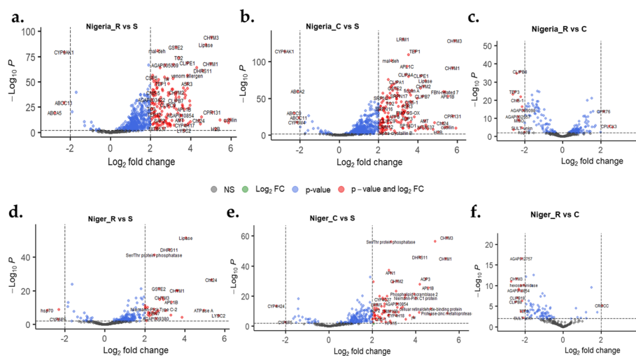
Fig. 1. A volcano plot of differentially expressed genes showing fold changes and levels of significance in R-S, C-S and R-C comparisons, for Nigeria and Niger populations of An. coluzzii . The plot depicts the top upregulated and top downregulated genes for each comparison, with several genes including chymotrypsins, a malate dehydrogenase, CYP450s, a glutathione S-transferase ( GSTe2 ), and a lipase, commonly upregulated in R vs S and C vs S comparisons. R stands for the female, resistant mosquitoes (survivors of 0.05% deltamethrin, 24 h after exposure), C stands for control (mosquitoes from the same population and of the same age not exposed to deltamethrin), and S stands for susceptible (females from fully insecticide-susceptible colony, Ngoussou)
