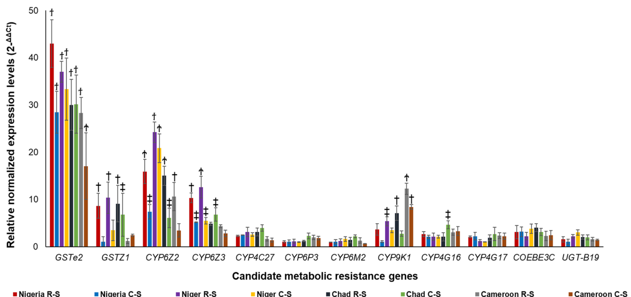
Fig. 3. Validation of candidate resistance genes. qRT-PCR profile of twelve metabolic resistance genes (in R-S and C-S comparisons) from the Sahelian An. coluzzii . Each bar (data point) is analysis from three biological replicates and three technical replicates for each gene, with error bars representing standard deviations. Significant differences are also indicated with the symbols †, ‡, † and ‡, for p < 0.0001 , p < 0.001 , p < 0.01 and p < 0.05 , respectively
