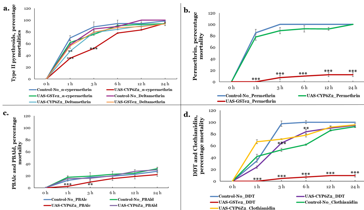
Fig. 6. Validation of the role of metabolic resistance genes in insecticide resistance. Results of insecticide susceptibility bioassays with transgenic flies expressing GSTe2 and CYP6Z2 . a \alpha -cypermethrin and deltamethrin, b permethrin, c 3-phenoxybenzaldehyde and 3-phenoxybenzyl alcohol, d DDT and clothianidin
