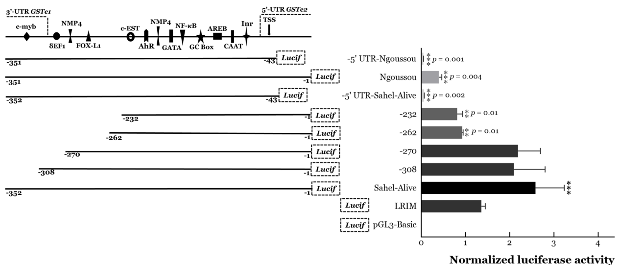
Fig. 5. Characterization of intergenic region (5' regulatory element) of GSTe2 . Results of dual luciferase reporter assays of the promoter (intergenic region) constructs, showing progressive loss of activity following sequential deletion of the constructs
