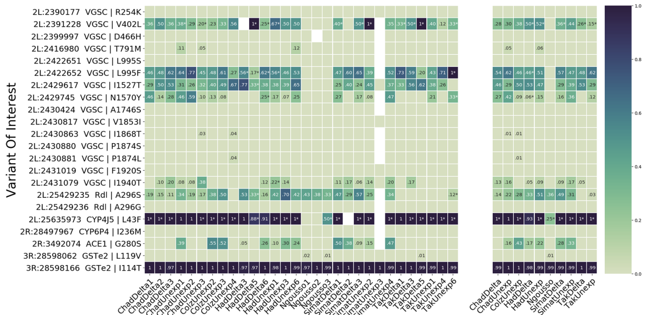
Fig. 4. Identification of resistance variants of interest. A heatmap showing frequencies of the resistance variants (haplotypes) in some key genes of interest
