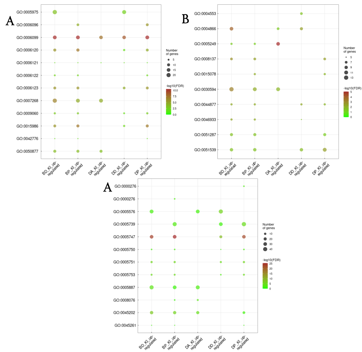
Additional file 13: Gene ontology enrichments Panel A shows enriched terms within biological process; B, the enriched terms in molecular functions and C, the cellular components.
