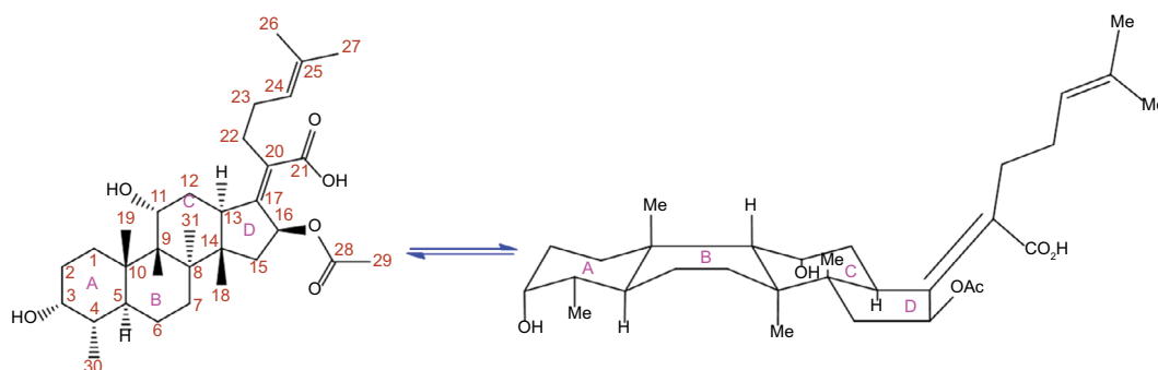
Figure 1 Chemical structure and conformation of fusidic acid (WU-FA-00).
