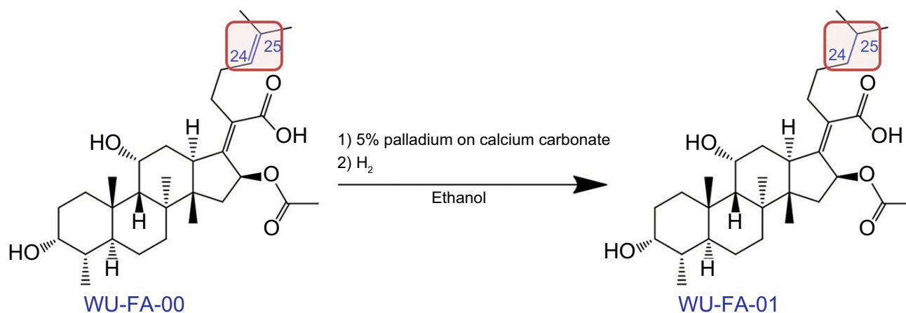
Scheme 1 Synthesis of the hydrogenation derivative of fusidic acid (WU-FA-01).
